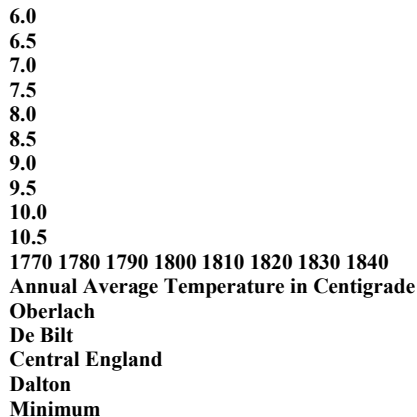
Figure 11: The Dalton Minimum in Europe
